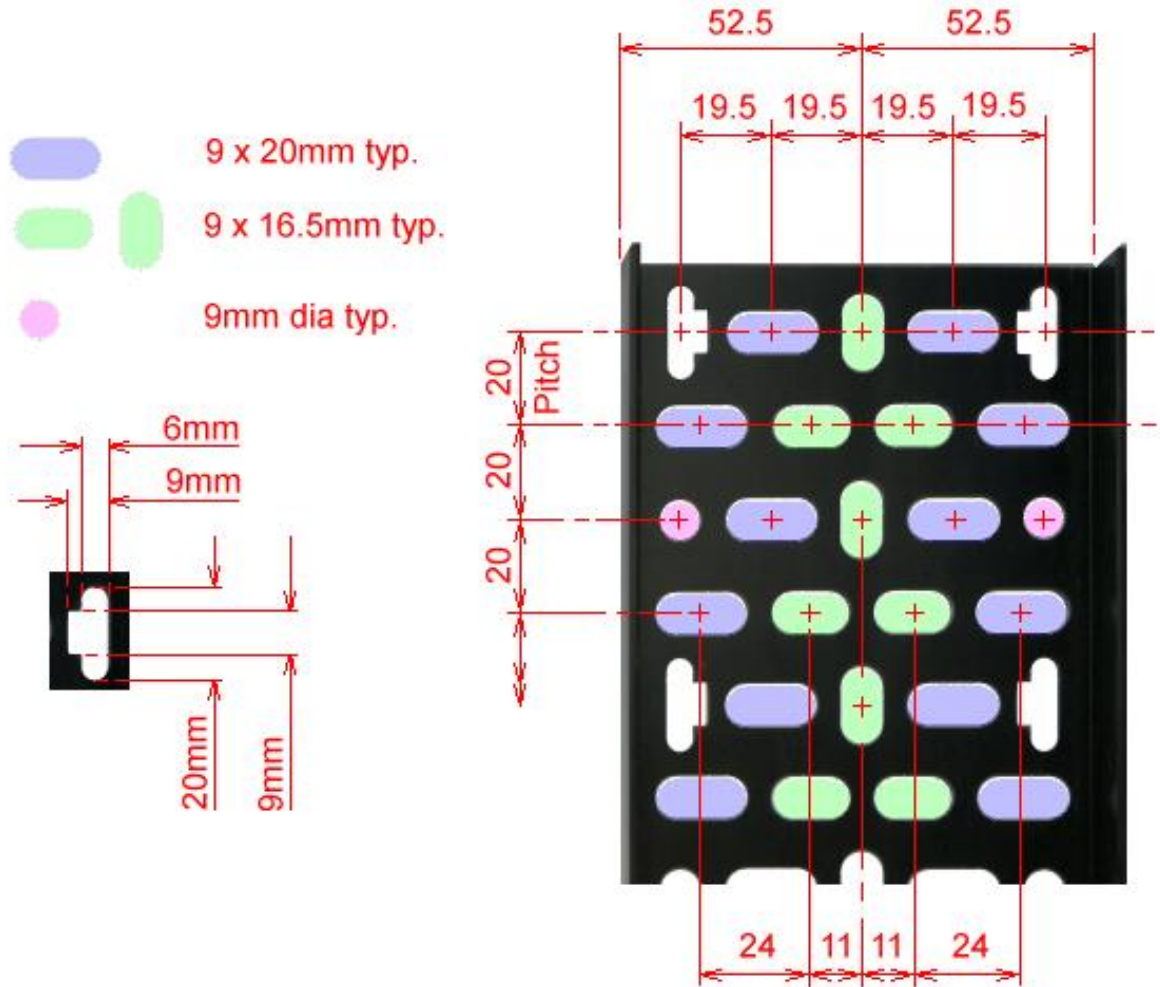
Canford plastic cable tray 105mm x 17mm x 2.5mm thk Supplied in 2m lengths
